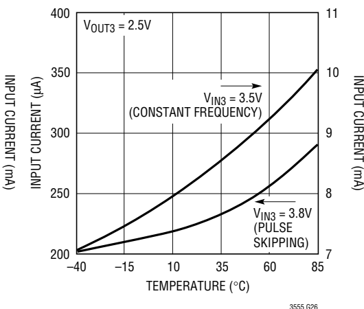
Switching Regulator 3 Pulse Skip Mode Quiescent Currents
