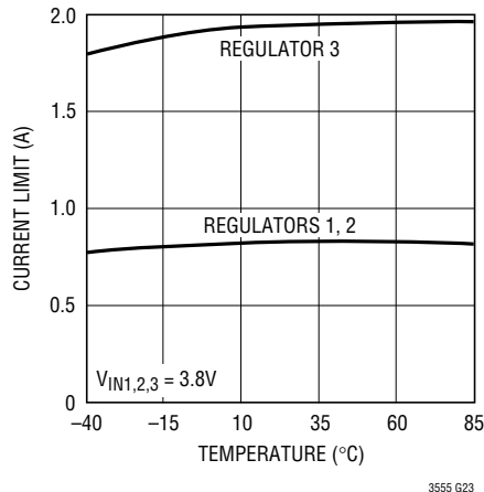
Switching Regulator Current Limit vs Temperature
